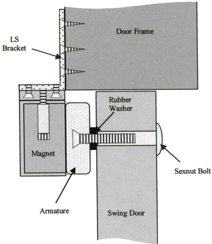
MOUNTING ON SWING DOOR WITH LS BRACKET WHERE THE HEADER IS TOO NARROW
