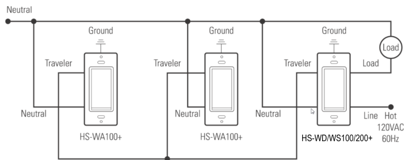
4-way circuit
