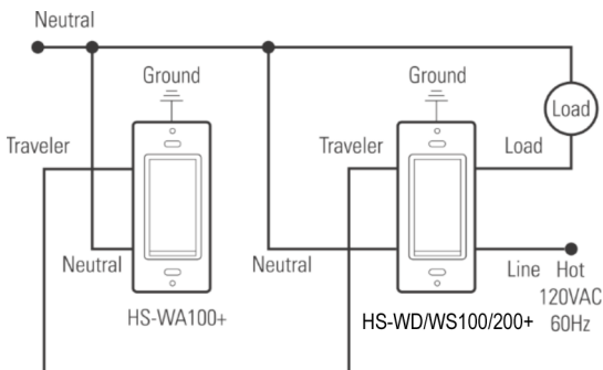
3-way circuit
